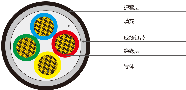
VV3+1芯电缆
