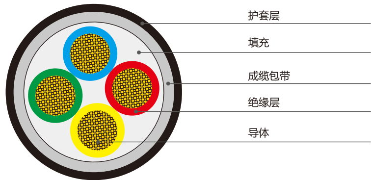
VV3+1芯电缆
