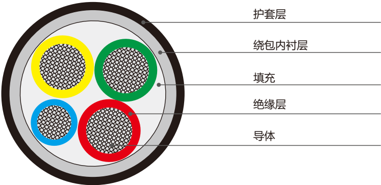
VV3+1芯电缆
